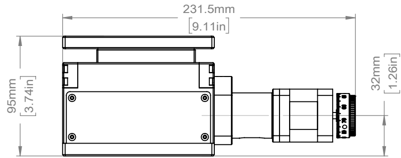
FULLY EXTENDED
